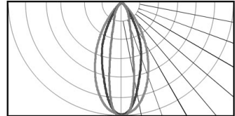
XS Model - Specular Reflector:
