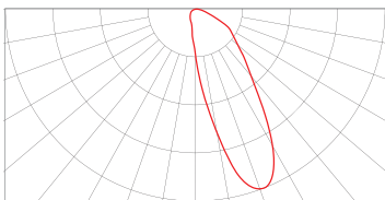
Wallwashing Optic (WW)
