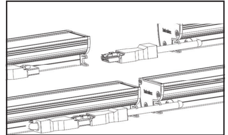
1. Align light fixtures next to each other and connect lights by using the 'PLUG + GO' system.
